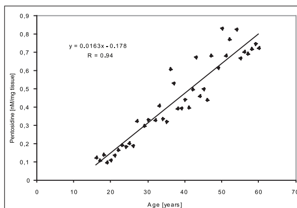
Fig. 3. The values of pentosidine amount in the tissue of intervertebral disc from persons between the ages of 16 and 60 years.
