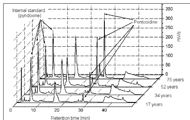
Fig. 1. Chromatograms of HPLC separation of hydrolyzates of intervertebral discs tissue. Peaks of pentosidine in persons of different age.
