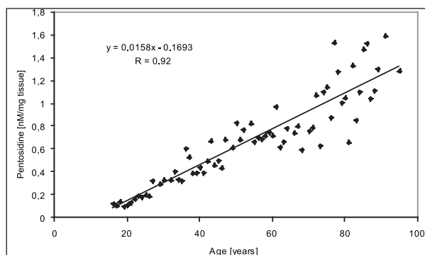
Fig. 2. The values of pentosidine amount in the tissue of intervertebral disc from persons between the ages of 16 and 95 years.
