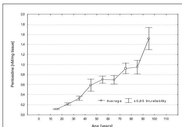
Fig. 4 The average amount of pentosidine in the tissue of intervertebral disc with limits of interval of reliability in age groups from second to tenth decade of life. It follows from the graph that age estimation by assessment of pentosidin in the tissue of intervertebral disc is reliable within the range of 15 to 40 years of age.
