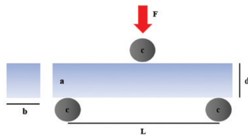
Fig. 4 Three points bending test
