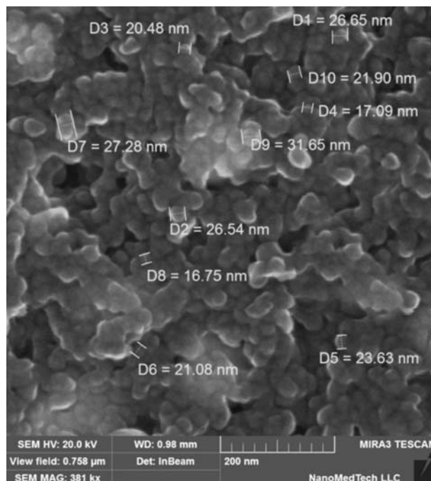
Fig. 6. A picture of Ag@Fe 3 O 4 nanoparticles using an electron microscope
