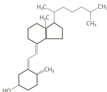
Cholekalciferol
