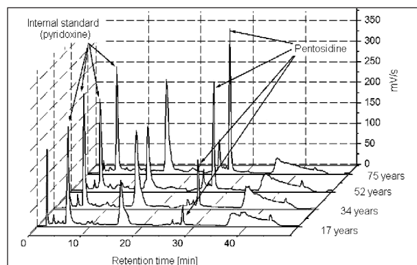
Fig. 1. Chromatograms of HPLC separation of hydrolysates of intervertebral discs tissue. Peaks of pentosidine in persons of different age.
