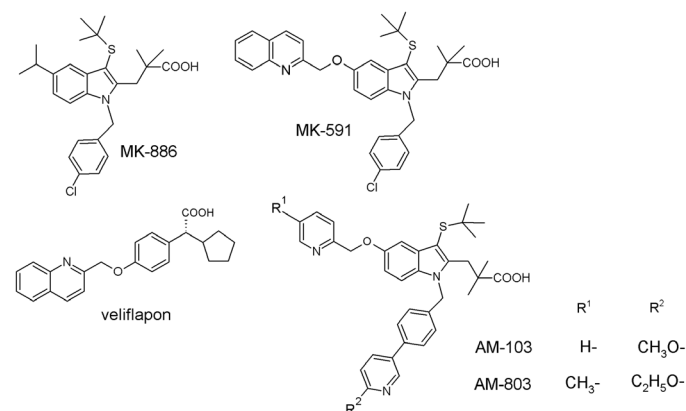
Obr. 4. FLAP inhibitory
