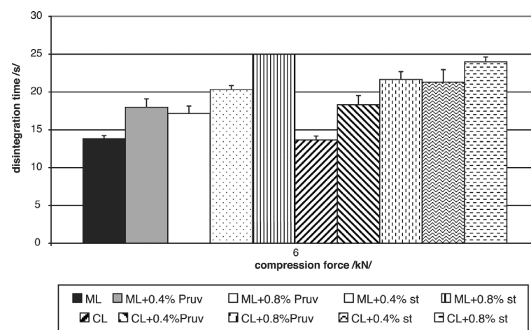
Fig. 4. Disintegration time of tablets – MicroceLac®100 and Cellactose®80 without and with Pruv and magnesi stearas
